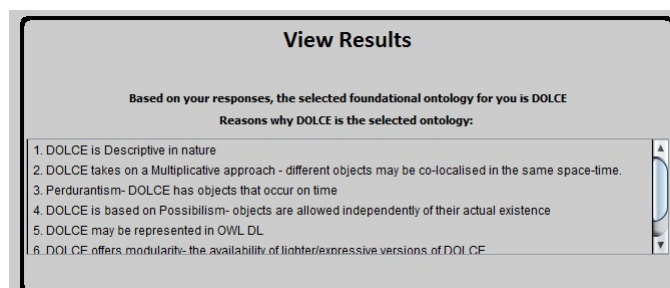
Figure 1: Output of ONSET: Scenario 1
